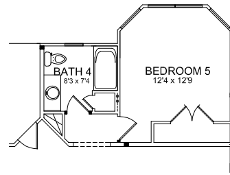
OPTIONAL BEDROOM 5 AND BATH 4
