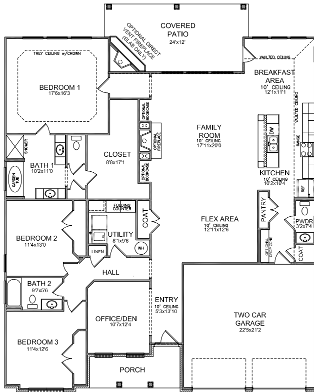
FIRST FLOOR PLAN A
