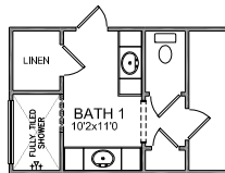
OPTIONAL BATH 1 LAYOUT SHOWN WITH 6'0"x3'8" FULLY TILED SHOWER. VANITY AT SHOWER CHANGES FROM 5' TO 6' SINGLE BOWL
