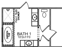
OPTIONAL BATH 1 LAYOUT SHOWN WITH 36x72 DROP IN GARDEN TUB AND 4'0"x3'4" FULLY TILED SHOWER.
