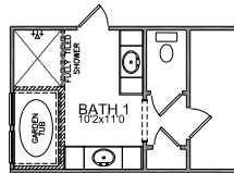
OPTIONAL BATH 1 LAYOUT SHOWN WITH 42x72 DROP IN GARDEN TUB AND 4'6"x4'0" FULLY TILED SHOWER. VANITY AT TUB CHANGES FROM 5' TO 6' SINGLE BOWL
