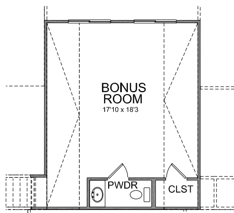
BONUS ROOM LAYOUT w/PWDR ROOM
