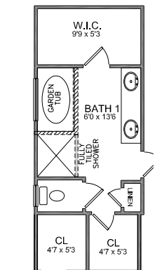
OPTIONAL BATH 1 SHOWN WITH 42x72 DROP IN GARDEN TUB, 4'x3'10" FULLY TILED SHOWER w/GLASS RETURN PANEL.
