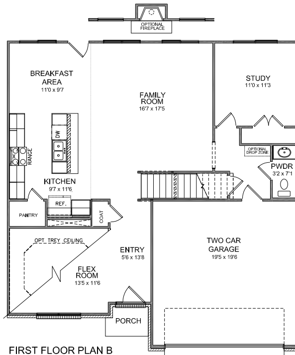
FIRST FLOOR PLAN B
