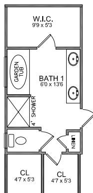
OPTIONAL BATH 1 SHOWN WITH 36x72 FLAT FRONT GARDEN TUB, 4' FIBERGLASS SHOWER.
