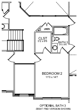
OPTIONAL BATH 3 (BSMT FND VERSION SHOWN)
