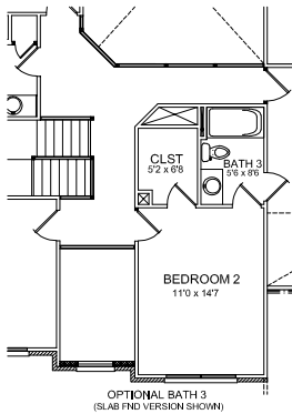
OPTIONAL BATH 3 (SLAB FND VERSION SHOWN)
