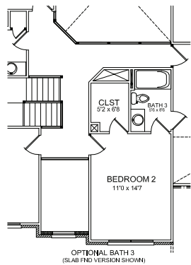
OPTIONAL BATH 3 (SLAB FND VERSION SHOWN)
