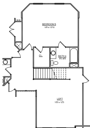
OPTIONAL BEDROOM 5 w/FULL BATH SHOWN w/ OPT LOFT
