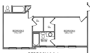
BEDROOM 3 & 4 SHOWN w/ OPTIONAL CLOSETS & OPTIONAL FULL BATH OVER ENTRY
