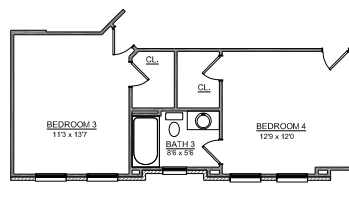
BEDROOM 3 & 4 SHOWN w/ OPTIONAL CLOSETS & OPTIONAL FULL BATH OVER ENTRY
