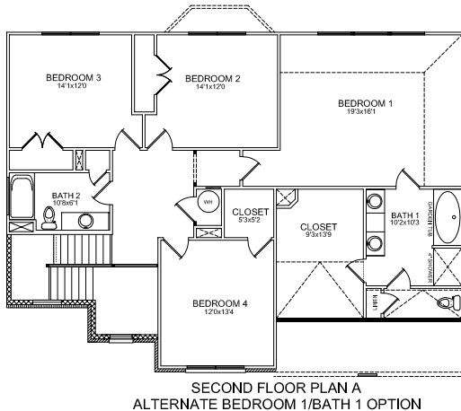
ALTERNATE BEDROOM 1/BATH 1 OPTION
