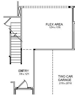
STAIRS FOR OPTIONAL BONUS ROOM LAYOUT
