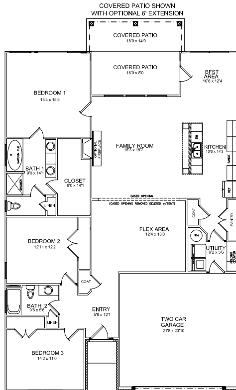
1ST FLOOR PLAN ELEV A ELEV B ELEV C
