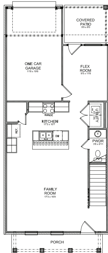
ELEVATION A FIRST FLOOR PLAN
