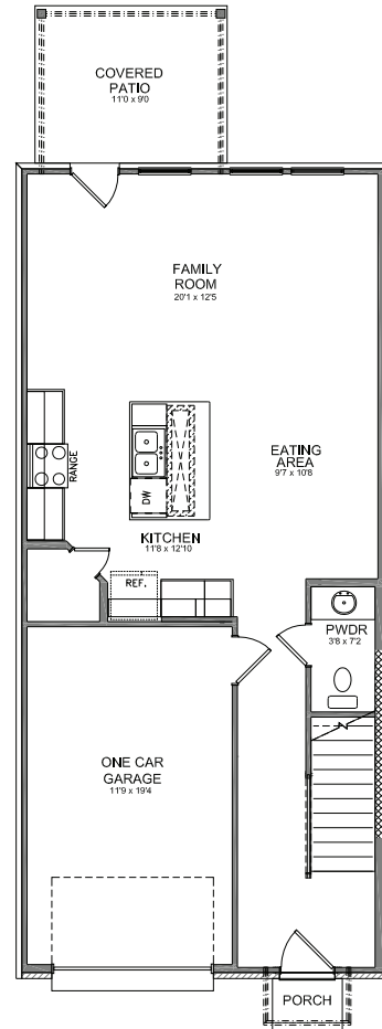
ELEVATION A FIRST FLOOR PLAN
