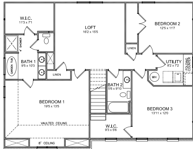
SECOND FLOOR PLAN A
