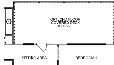
OPTIONAL COVERED DECK OFF BEDROOM 1 (REQUIRES ENLARGED PATIO OR DECK BELOW)
