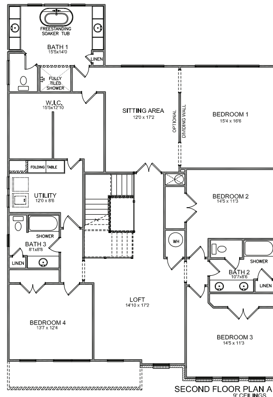
OPTIONAL COVERED DECK OFF BEDROOM 1 (REQUIRES ENLARGED PATIO OR DECK BELOW)
