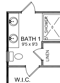
UPGRADED BATH 1 WITH 5'X3'6" SHOWER PAN W/TILED WALLS AND LINEN CLOSET
