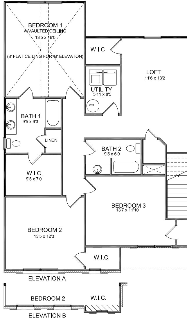
SECOND FLOOR PLAN KNOXVILLE AREA
