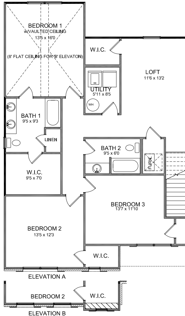
SECOND FLOOR PLAN KNOXVILLE AREA
