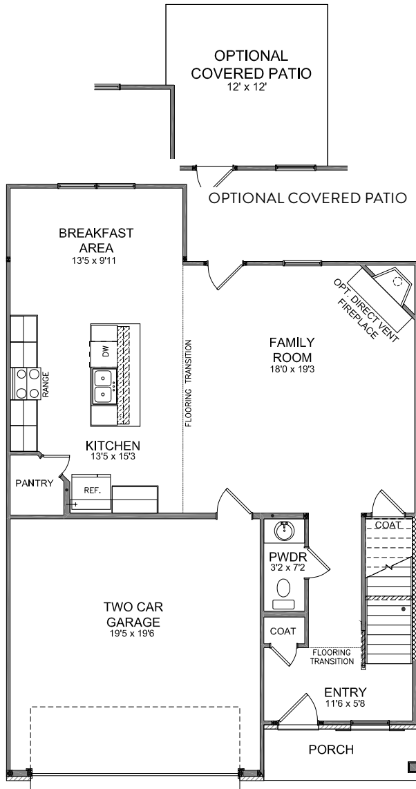
FIRST FLOOR PLAN CENTRAL KENTUCKY
