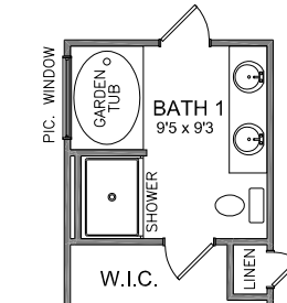
UPGRADED BATH 1 WITH 42X60 GARDEN TUB PICTURE WINDOW ABOVE 4'X3' FIBERGLASS SHOWER
