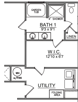
OPTIONAL BATH 1 W/42X60 GARDEN TUB & 4'X3' SHOWER
