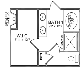
UPGRADED BATH 1 WITH 42X60 GARDEN TUB WITH PICTURE WINDOW ABOVE 4'X3' FIBERGLASS SHOWER
