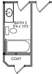
OPTIONAL 1ST FL. BATH 3 LAYOUT
