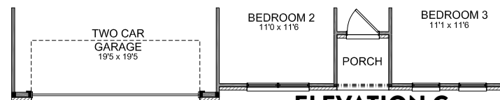
ELEVATION C
