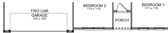
ELEVATION C FIRST FLOOR PLAN
