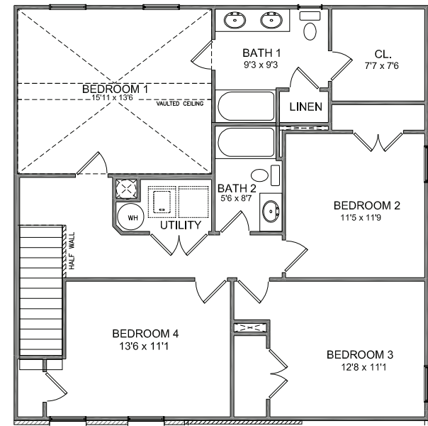
SECOND FLOOR SHOWN WITH OPTIONAL BEDROOM 4 IN LIEU OF LOFT
