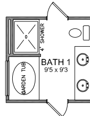
UPGRADED BATH 1 WITH 42X60 GARDEN TUB WITH PICTURE WINDOW ABOVE 4'X3' FIBERGLASS SHOWER
