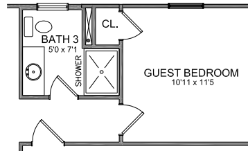
OPTIONAL GUEST BEDROOM, BATH 3 W/4' VANITY & 4'X3' FIBERGLASS SHOWER
