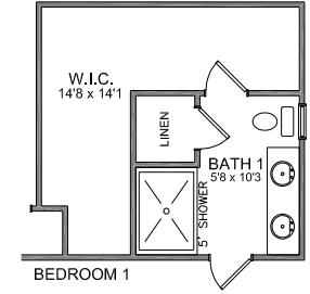
UPGRADED BATH 1 WITH 5'X3'6" SHOWER PAN W/TILED WALLS AND LINEN CLOSET
