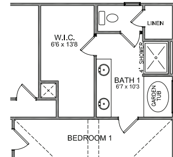
UPGRADED BATH 1 WITH 42X60 GARDEN TUB WITH PICTURE WINDOW ABOVE 4'X3' FIBERGLASS SHOWER
