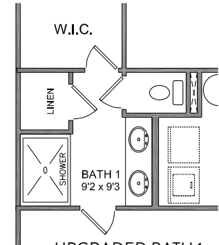
UPGRADED BATH 1 5'X3'6" SHOWER PAN W/TILED WALLS AND LINEN CLOSET
