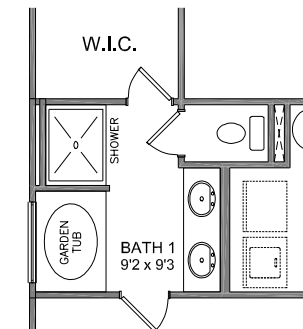
UPGRADED BATH 1 42X60 GARDEN TUB PICTURE WINDOW ABOVE & 4'X3' FIBERGLASS SHOWER
